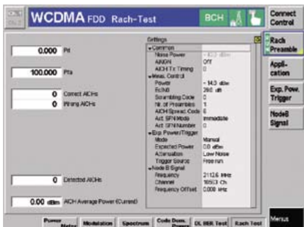
AICH analysis.
