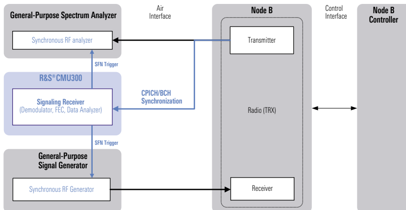
Test setup for synchronized measurements with general-purpose test equipment.
