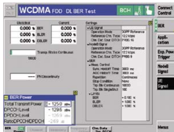
Downlink RMC data analysis (here, continuous measurement with averaging over 10 000 transport blocks).
