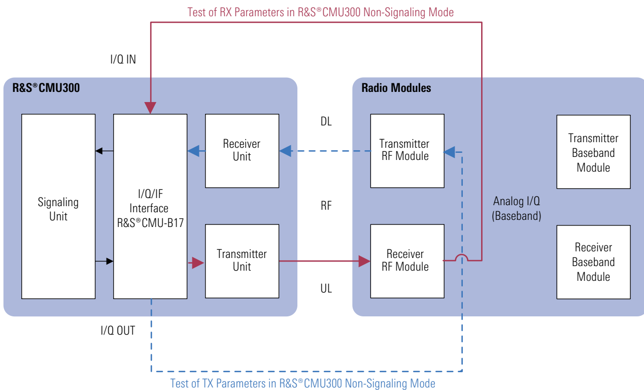
Signal paths when testing RF modules.
