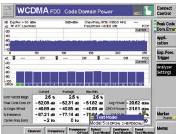
Peak Code Domain Error (PCDE) measurement on a HSDPA test model.
