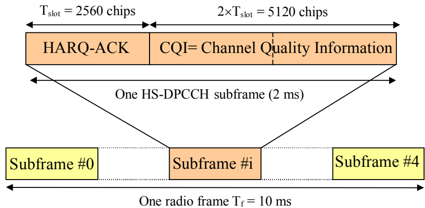
Figure 4 – Structure of HS-DPCCH
