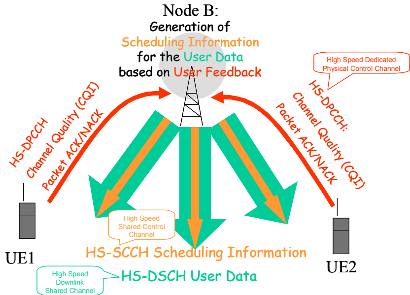
Figure 1 – HSDPA Principle
