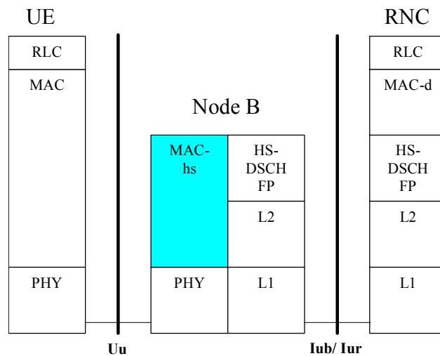
Figure 5 HSDPA Protocol Architecture
