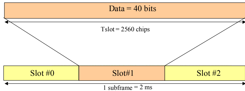
Figure 3 –Structure of HS-SCCH
